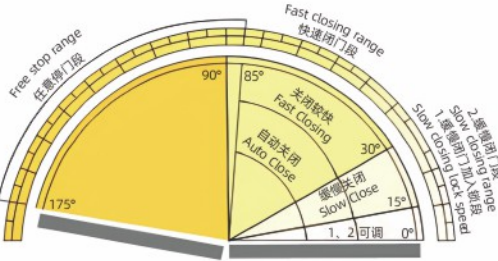
各门类定位功能示意图 Schematic diagram of each door segment positioning function
