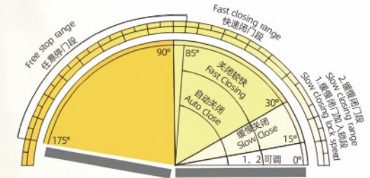
各门类定位功能示意图 Schematic diagram of each door segment positioning function
