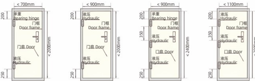
各门类定位功能示意图 Schematic diagram of each door segment positioning function
