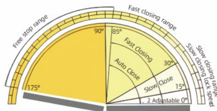
Schematic diagram of each door segment positioning function
